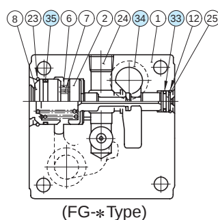
Section X-X
