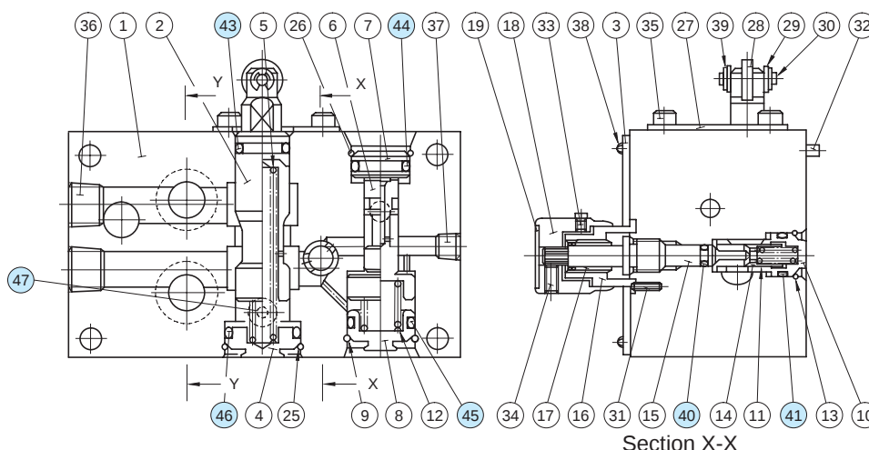
Section X-X
